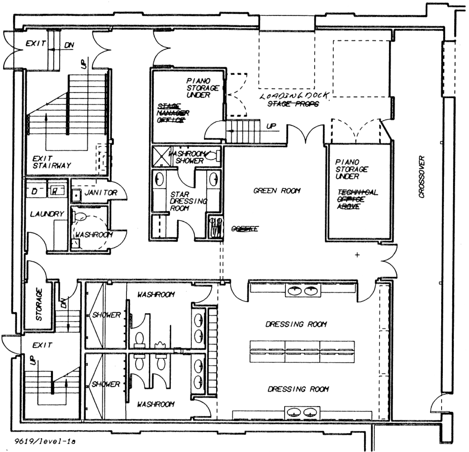
BACK STAGE (DRESSING ROOMS) SCALE 1:100
