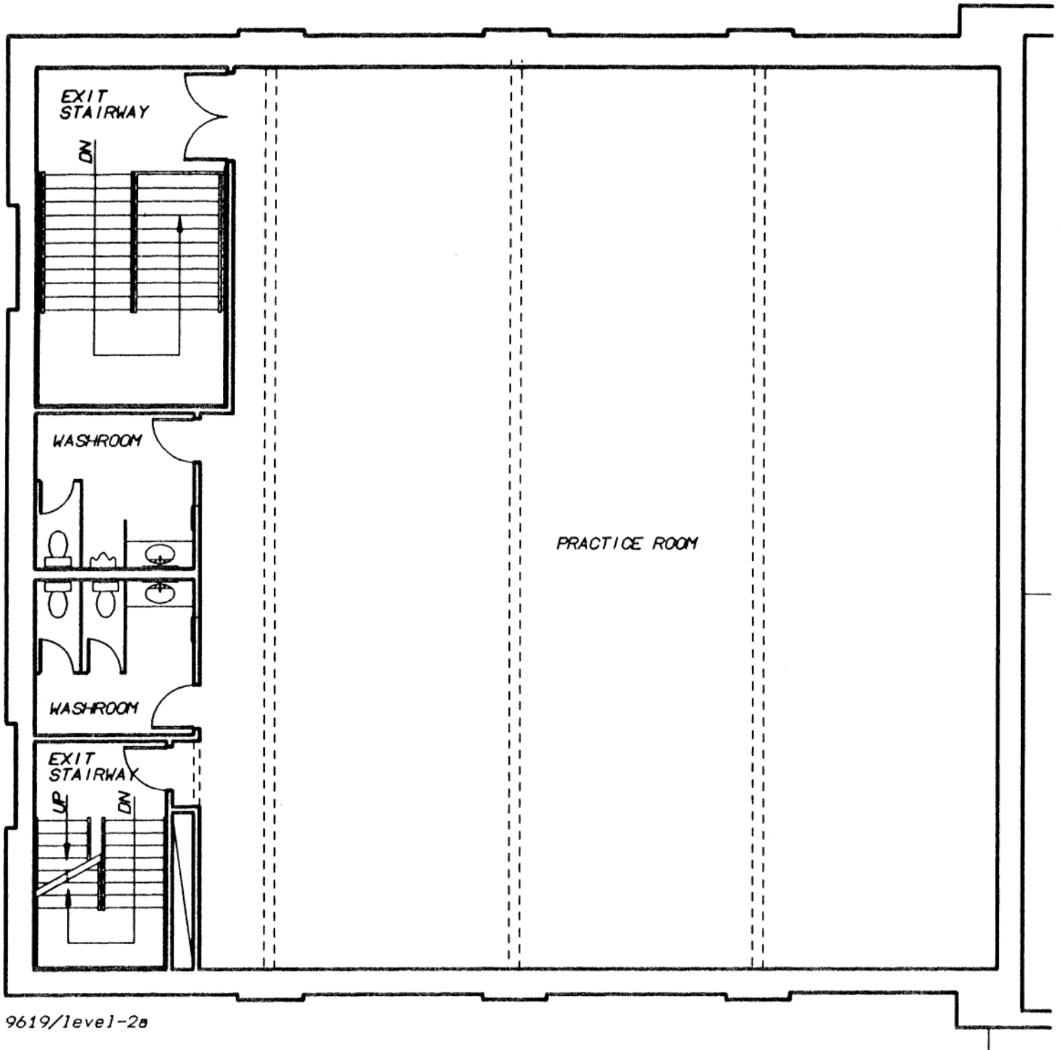
BACK STAGE (LEVEL-2 PRACTICE ROOM) SCALE 1:100
